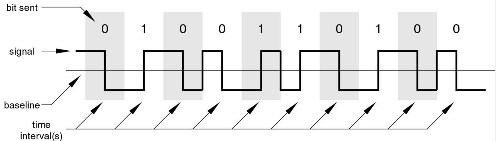
Manchester Encoding
